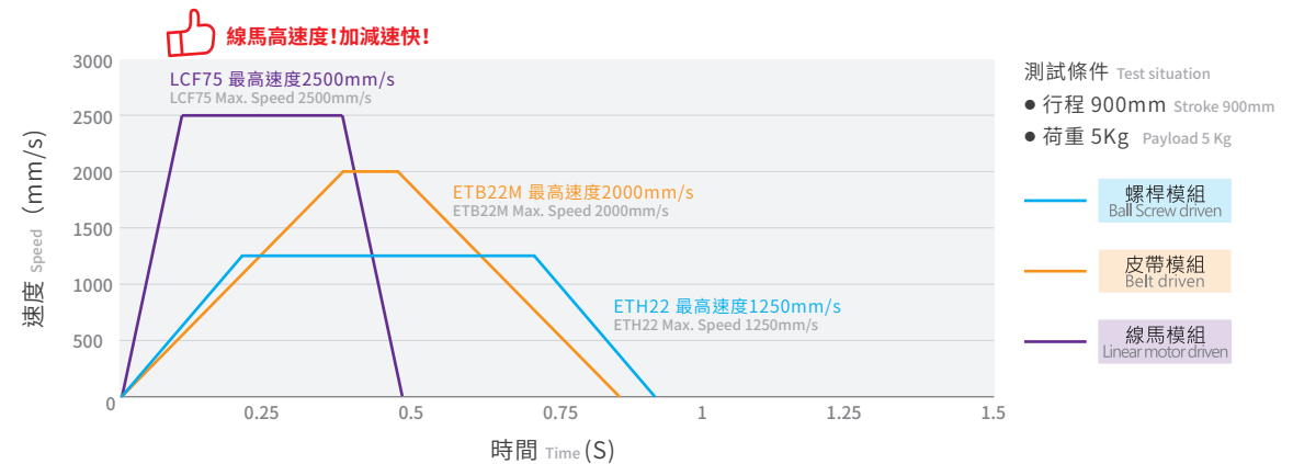
線馬模組與螺桿、皮帶模組移動速度比較 Speed comparison between linear motor and belt, ballscrew driven actuator.
